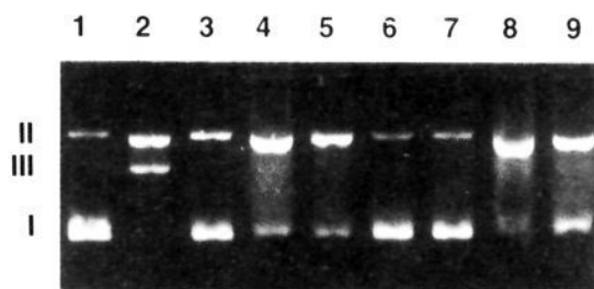
Figure 2. Strand scission of \phi X174 replicative form DNA. DNA samples (180 ng) in 40 \mu L of H 2 O containing 3% dimethoxyethane were treated as indicated below, incubated at 25 °C for 30 min, and then analyzed on a 1.2% agarose gel (40 V, 18 h). Lane 1, DNA alone; lane 2, 10 \mu M Fe(II) + 0.1% H 2 O 2 ; lane 3, 10 \mu M Cu(II); lane 4, 20 \mu g of a CH 2 Cl 2 extract of H. trifurcata + 10 \mu M Cu(II); lane 5, 10 \mu g of extract + 10 \mu M Cu(II); lane 6, 20 \mu g of hexane layer + 10 \mu M Cu(II); lane 7, 10 \mu g of hexane layer + 10 \mu M Cu(II); lane 8, 20 \mu g of aqueous methanol layer + 10 \mu M Cu(II); lane 9, 10 \mu g of aqueous methanol layer + 10 \mu M Cu(II).
